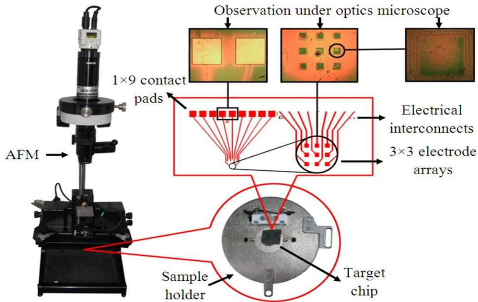
Fig. 3. Experimental setup for scanning and measurement based on AFM.
