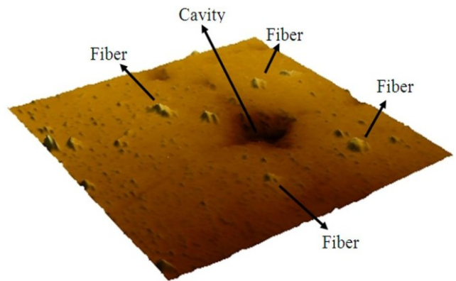
Fig. 6. A 3D image generated based on the 2D topography image as shown in Figure 5.
