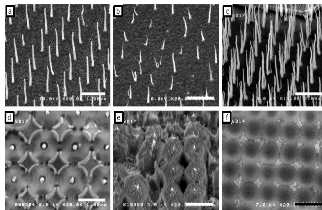
Fig. 2. Top row shows the importance of PECVD chamber conditioning on CNF growth: (a) final run in "warm chamber"; (b) initial run in "cold chamber"; (c) Effect of high thermal ramps (~200°C/min) resulting in multiple fibers from single nanopot. Bottom row illustrates SEM images of patterned arrays after re-exposing VACNF tips by Reactive Ion Etching (d), (e) and CMP (f). The dots are 100nm in diameter and 1µm in spacing.
