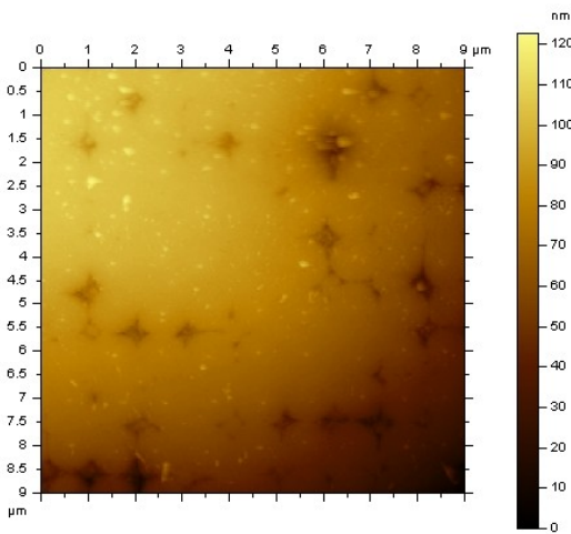
Fig. 4. Topography scan image of array 1 in 9\mu\text{m} square area: cavities are located to zoom in for fibers.
