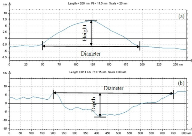
Fig. 7. Cross-section information for measurement based on the line crossing (a) a fiber and (b) a cavity in Figure 6.
